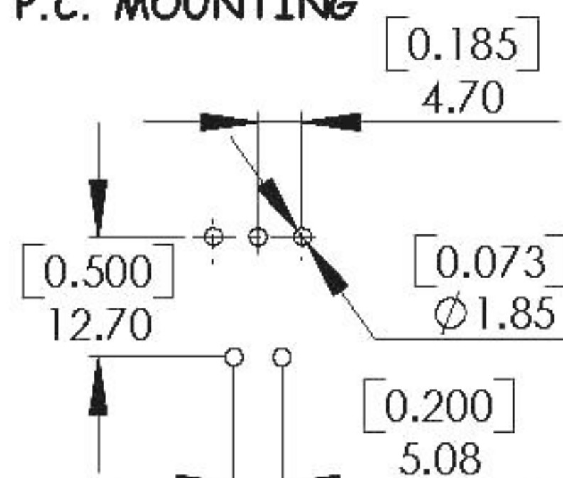
P.C. MOUNTING
