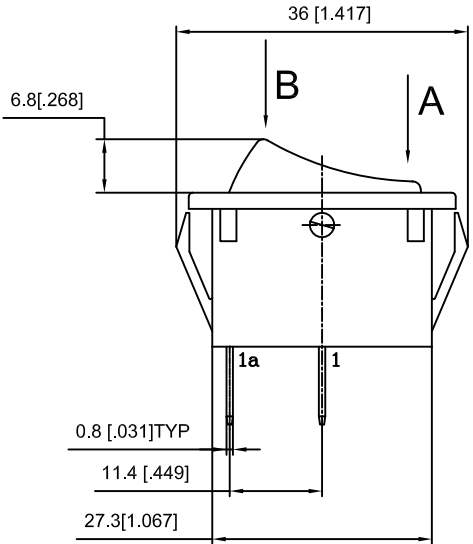
CIRCUIT SPST
