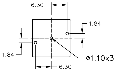
P.C. MOUNTING
