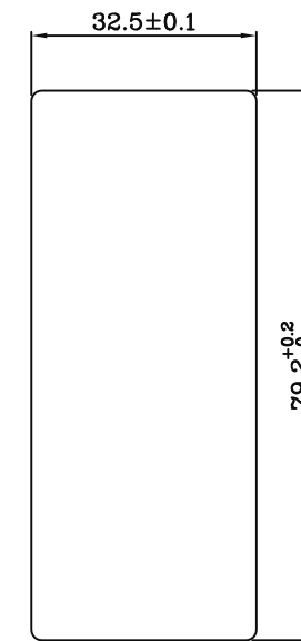
PANEL CUT-OUT
