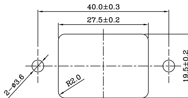
PANEL CUT-OUT
