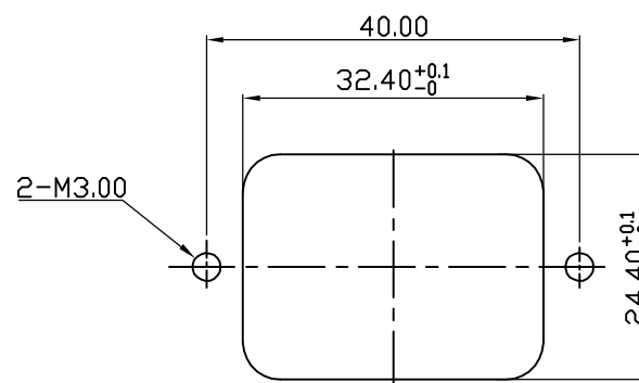
PANEL CUT-OUT
